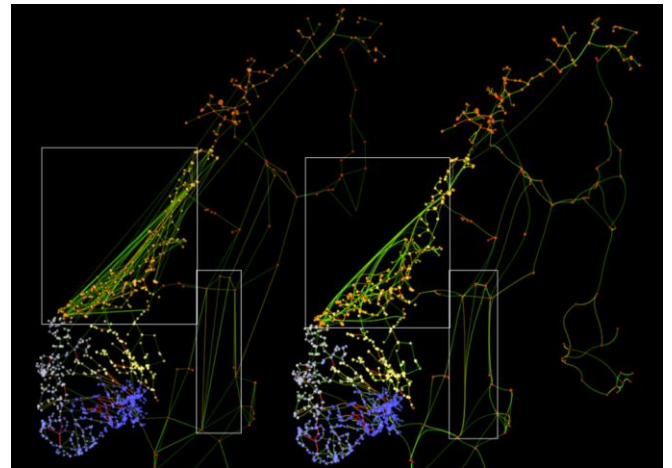
Figure 4: Demonstration of normal visualization (left) and edge bundling (right) on the power net of Norway. Extra edges have been added in the large box for demonstration purposes.
